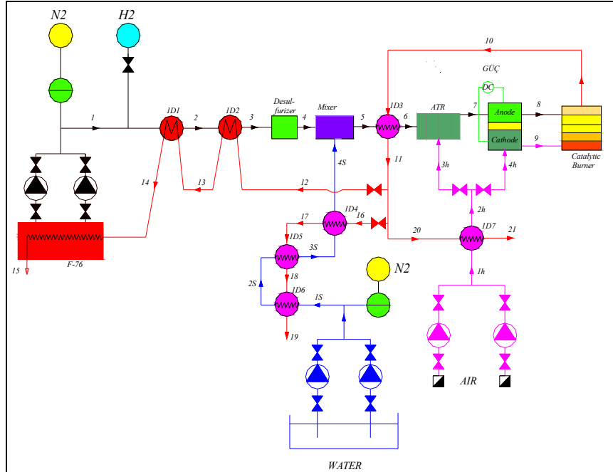
Fig.5. Diesel-fueled SOFC system
