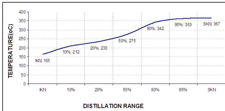
Fig. 4. A Typical of distillation curve of F-76 diesel fuel
